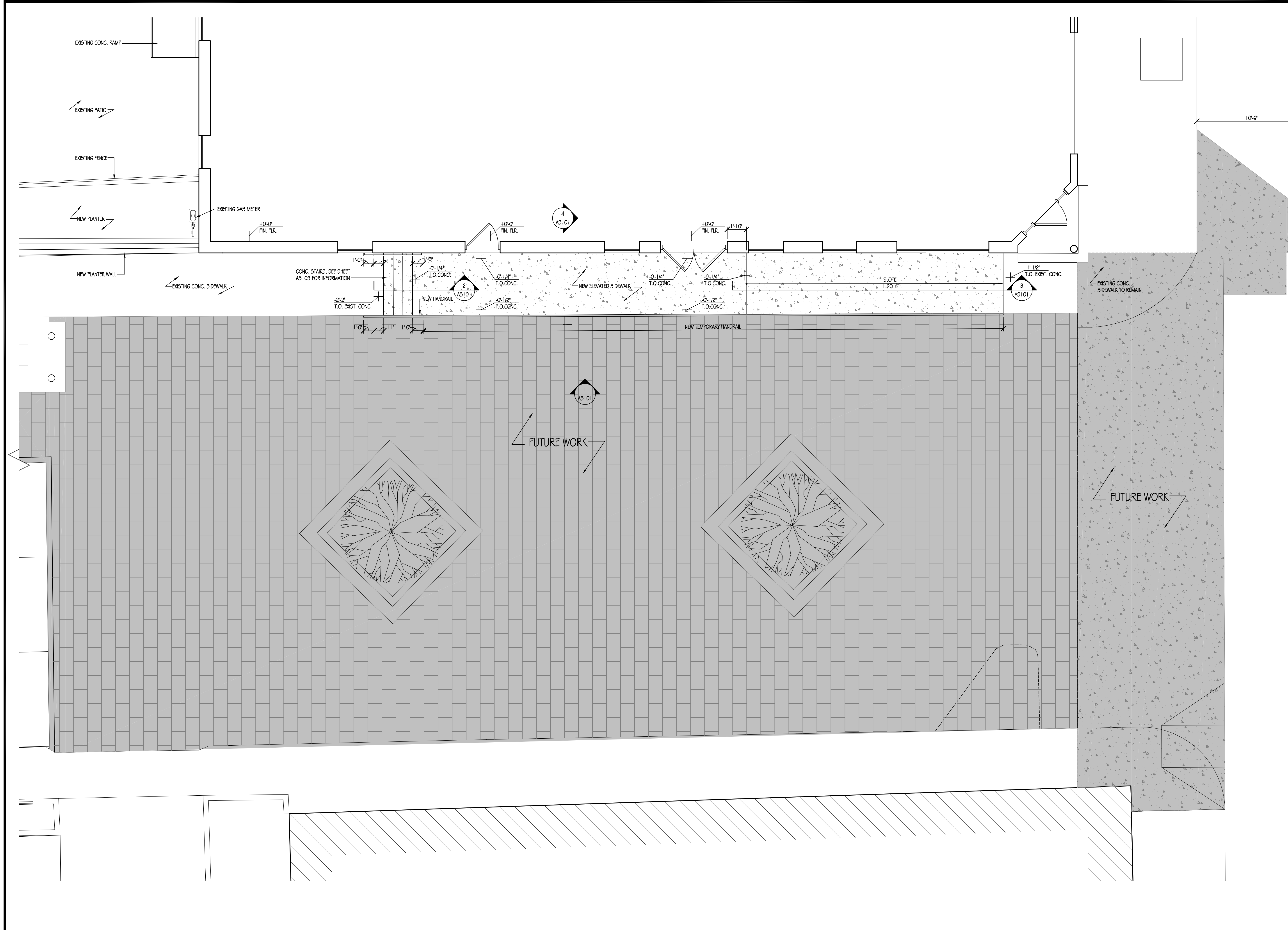
SIDEWALK PLAN SCALE: 1/4" = 1'-0"
